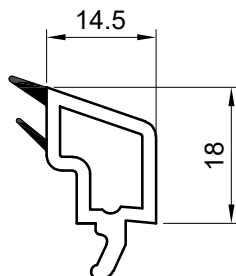
508006-231 Junquillo 14.5 Blanco 508006-233 Junquillo 14.5 Beige 508006-236 Junquillo 14.5 Clay
