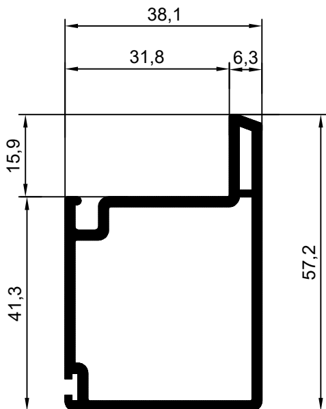
201605-231 Hoja Jamba 2090 blanco 201605-233 Hoja Jamba 2090 beige 201605-236 Hoja Jamba 2090 clay
