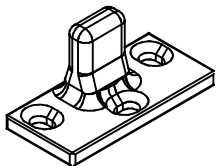
329025-001 FLUSH I-BOLT (Cerradero de marco Invisifold)
